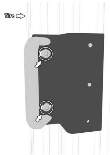
Fig.6: Attach the mounting plate with the anchor plate to the profile and align with the process guard locking. Tighten the Torx screws M8 x 12 mm.
